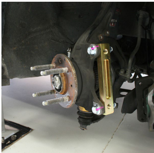
Figure 1: Older version bracket shown
