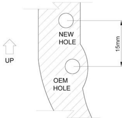
Figure 2: Pedal after modification. Ensure clevis can rotate freely +/- 20 deg about the horizontal position once pedal is reinstalled.
