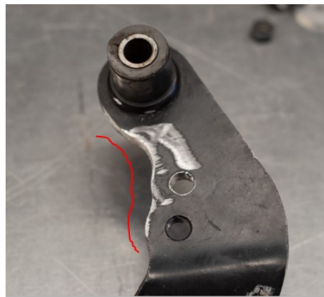
Figure 2: Pedal after modification. Ensure clevis can rotate freely +/- 20 deg about the horizontal position once pedal is reinstalled.
